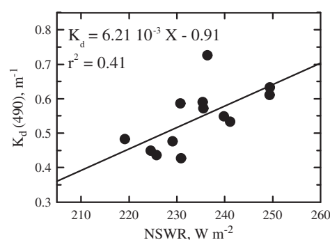
Fig. 8. Relationship between monthly vertical diffuse attenuation coefficient K_d(490) and net shortwave radiation flux (NSWR) in the Baltic Sea in the month of July.
