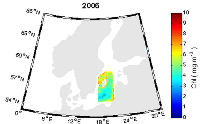
Fig. 1. Location of our study area in the Baltic Sea. Color scale indicates annual concentration of surface chlorophyll (Chl) derived from SeaWiFS data in 2006.
