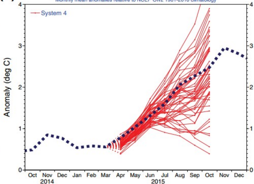
(b) NINO3.4 SST anomaly plume ECMWF forecast from 1 Apr 2015 Monthly mean anomalies relative to NCEP OIv2 1981-2010 climatology
