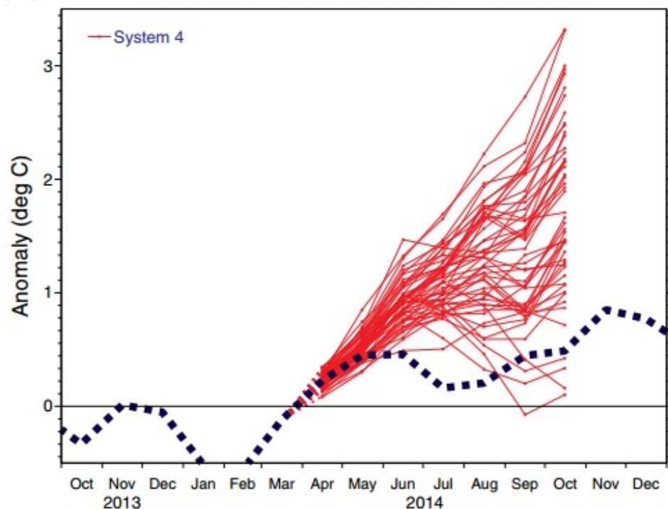
(a) NINO3.4 SST anomaly plume ECMWF forecast from 1 Apr 2014 Monthly mean anomalies relative to NCEP OIv2 1981-2010 climatology
