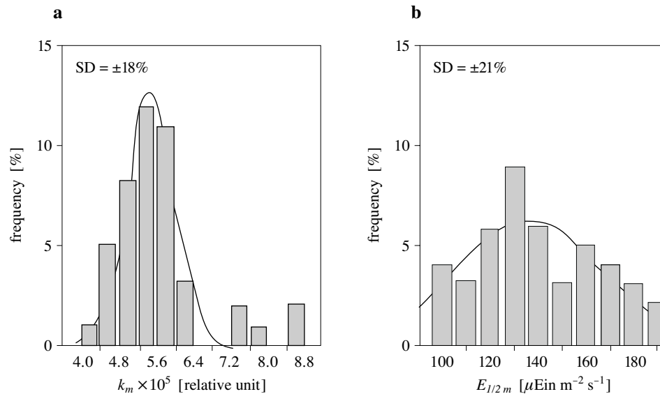
Fig. 2. Histograms of k_m (a) and E_{1/2m} (b) distribution, determined for the Baltic Sea stations
