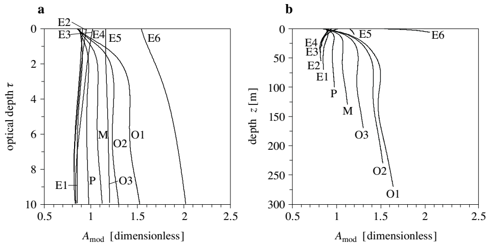
Fig. 6. Computed (using the model according to Ostrowska 2000) depth profiles of the ratio A_{mod} = \tilde{a}_{pl, PSP} / \tilde{a}_{pl, PSP, fl} for optical (a) and real (b) depths for different trophic types of sea. Surface chlorophyll a concentrations C_a(0) [mg tot.chl a m^{-3} ] were assumed to represent the water trophic type index (according to Woźniak et al. 1992): O1 - C_a(0) = 0.035 ; O2 - C_a(0) = 0.07 ; O3 - C_a(0) = 0.15 ; M - C_a(0) = 0.35 ; P - C_a(0) = 0.7 ; E1 - C_a(0) = 1.5 ; E2 - C_a(0) = 3.5 ; E3 - C_a(0) = 7 ; E4 - C_a(0) = 15 ; E5 - C_a(0) = 35 ; E6 - C_a(0) = 70
