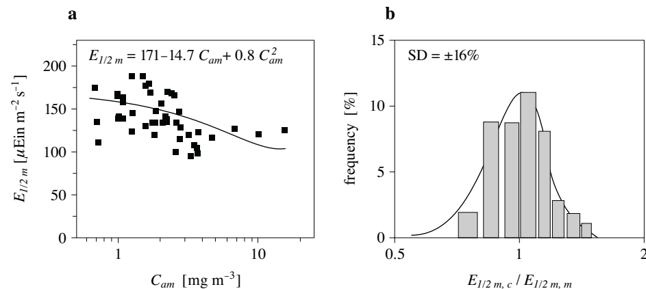
Fig. 4. The dependence of E_{1/2m} on the chlorophyll a C_{am} content averaged over the water column and polynomial regression of this dependence (a); histogram of distribution of the ratio of E_{1/2m,c}/E_{1/2m,m} (index c – calculated, using polynomial regression values of E_{1/2m} , index m – observed values of this parameter) (b)
