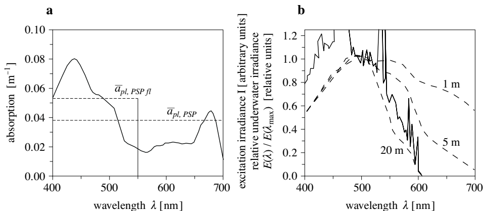
Fig. 1. Exemplary spectrum of phytoplankton light absorption coefficient from the central Baltic Sea. Values of absorption coefficients are averaged over the 400–550 nm ( \bar{a}_{pl, PSP, fl} ) and 400–700 nm ( \bar{a}_{pl, PSP} ) spectral regions (a). Spectrum of the light used to excite chlorophyll fluorescence in the PrimProd fluorometer (solid line), and spectral distributions of underwater irradiance in the sea at different depths (dashed lines – data by M. Ostrowska and R. Hapter) (b)
