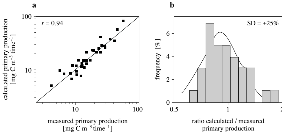
Fig. 5. Dependence of the calculated primary production of phytoplankton on the measured value averaged over the water column at Baltic Sea stations (a), histogram of the distribution ratio of the calculated productions to the measured values (b)
