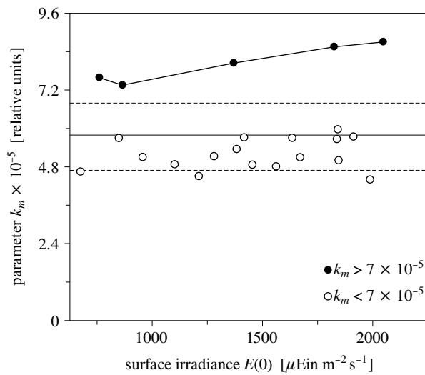
Fig. 3. Dependence of k_m on surface irradiance E(0) for the Baltic Sea stations. Dashed lines show the standard deviation band
