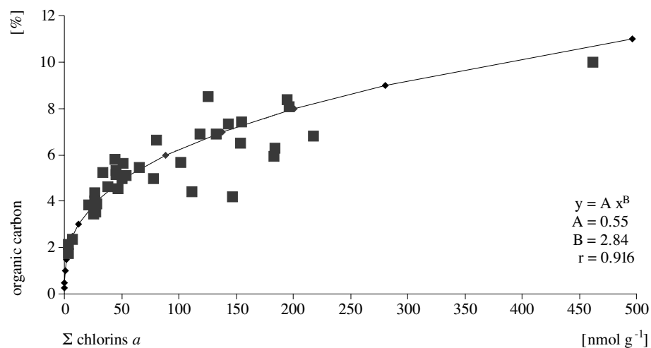
Fig. 11. Plot of the sum of major chlorins a [nmol g -1 ] vs organic carbon [%]
