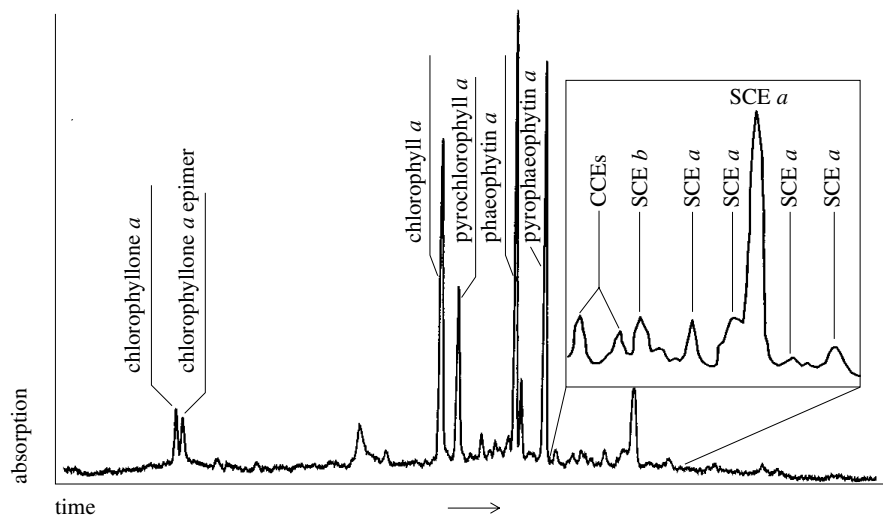
Fig. 4. HPLC–MS diode-array chromatogram (660 nm) of a Gotland Deep sediment extract (layer 68–72 cm)
