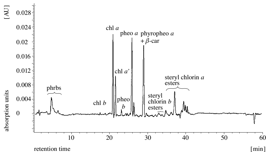
Fig. 2. Diode-array HPLC chromatogram (660 nm) of a Gotland Deep sediment extract (layer 68–72 cm)
