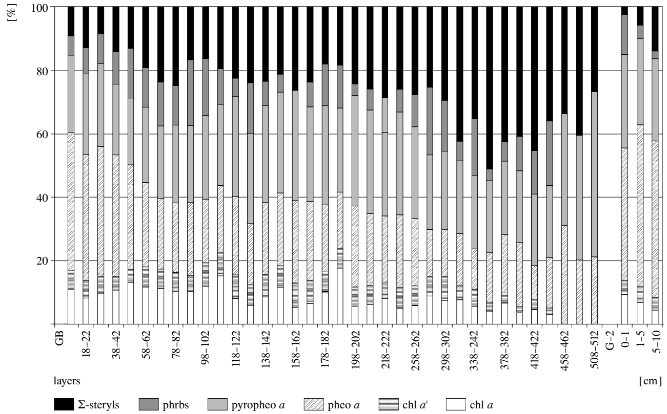
Fig. 10. Proportion [%] of major chlorins a [ \text{nmol g}^{-1} ] relative to the sum of chlorins a in the Gotland Deep (GB) and Gdańsk Deep (G-2) sediments (the short forms used in above legend are the same as those in the caption to Fig. 6)
