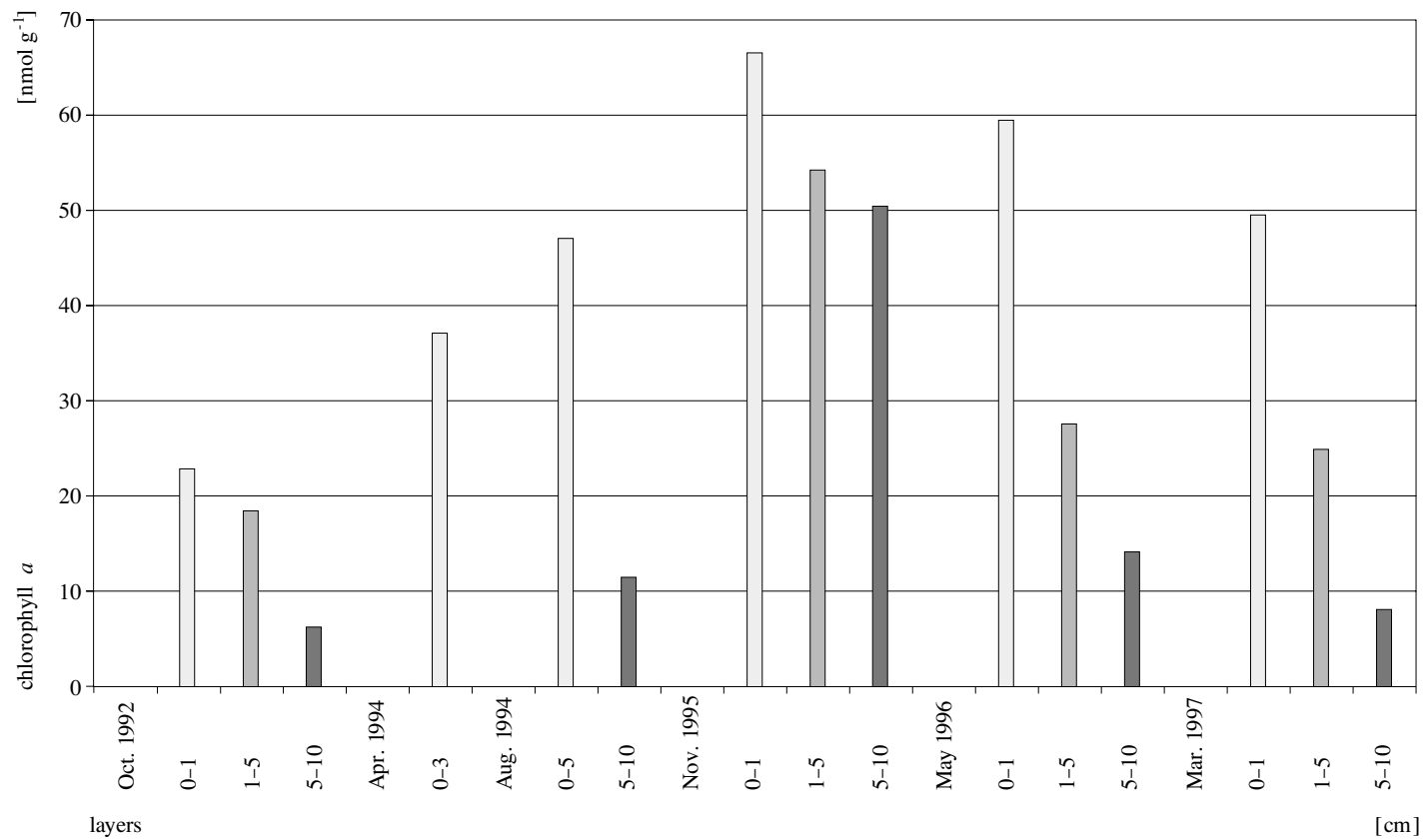
Fig. 9. Chlorophyll a concentrations in recent sediments from the Gdańsk Deep, collected in 1992–1997
