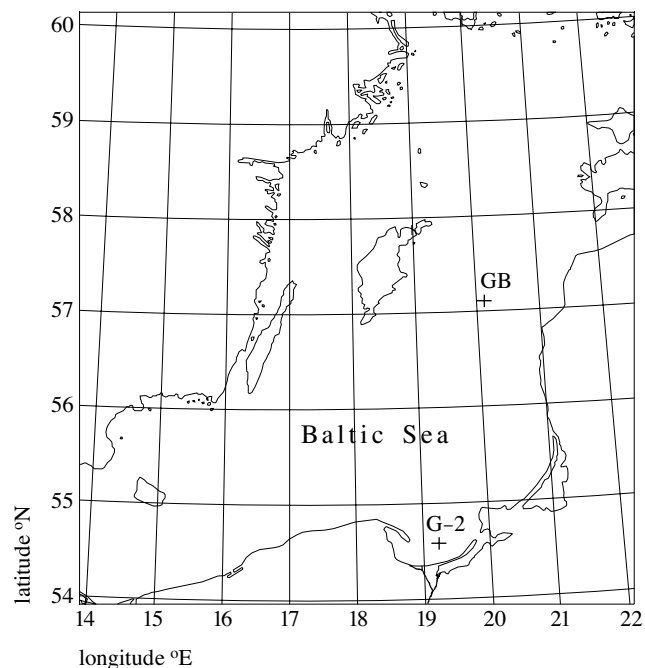
Fig. 1. Location of the sampling sites
