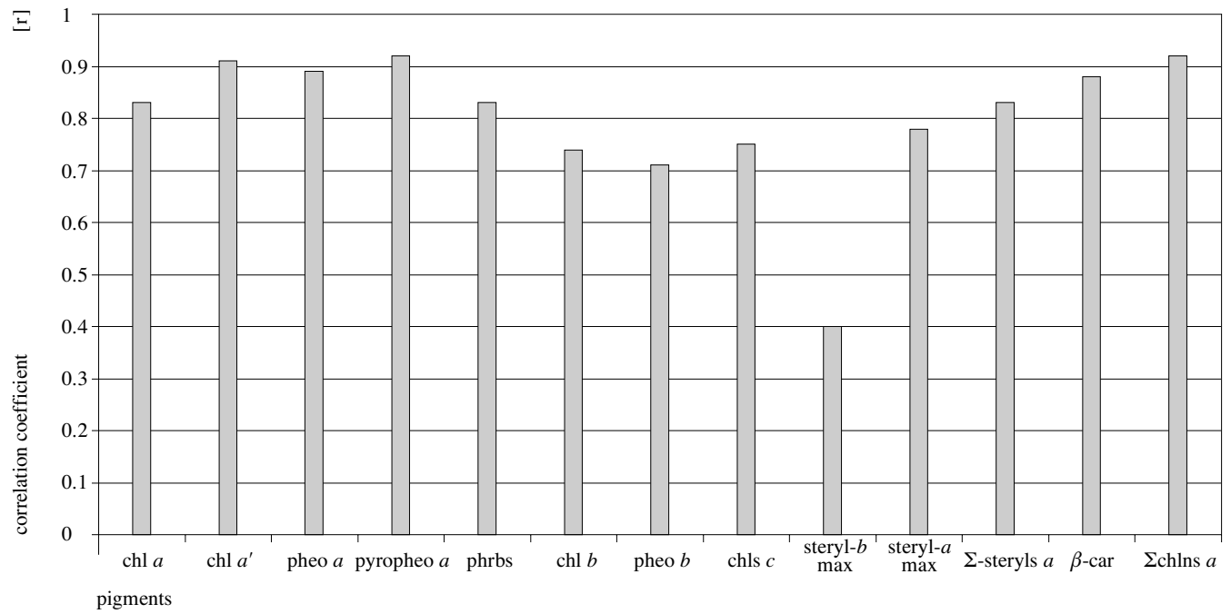
Fig. 12. Plot of exponential correlation coefficients of the determined pigments with organic carbon (the short forms used above are the same as those in the captions to Figs. 6 and 7)
