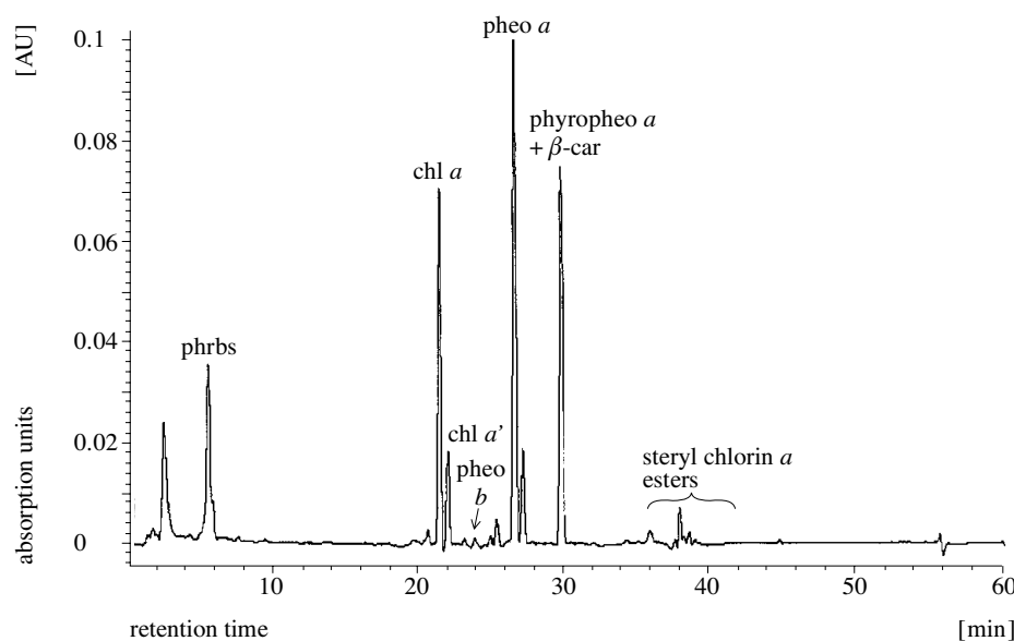
Fig. 3. Diode-array HPLC chromatogram (660 nm) of a recent (0–1 cm) sediment extract from the Gdańsk Deep
