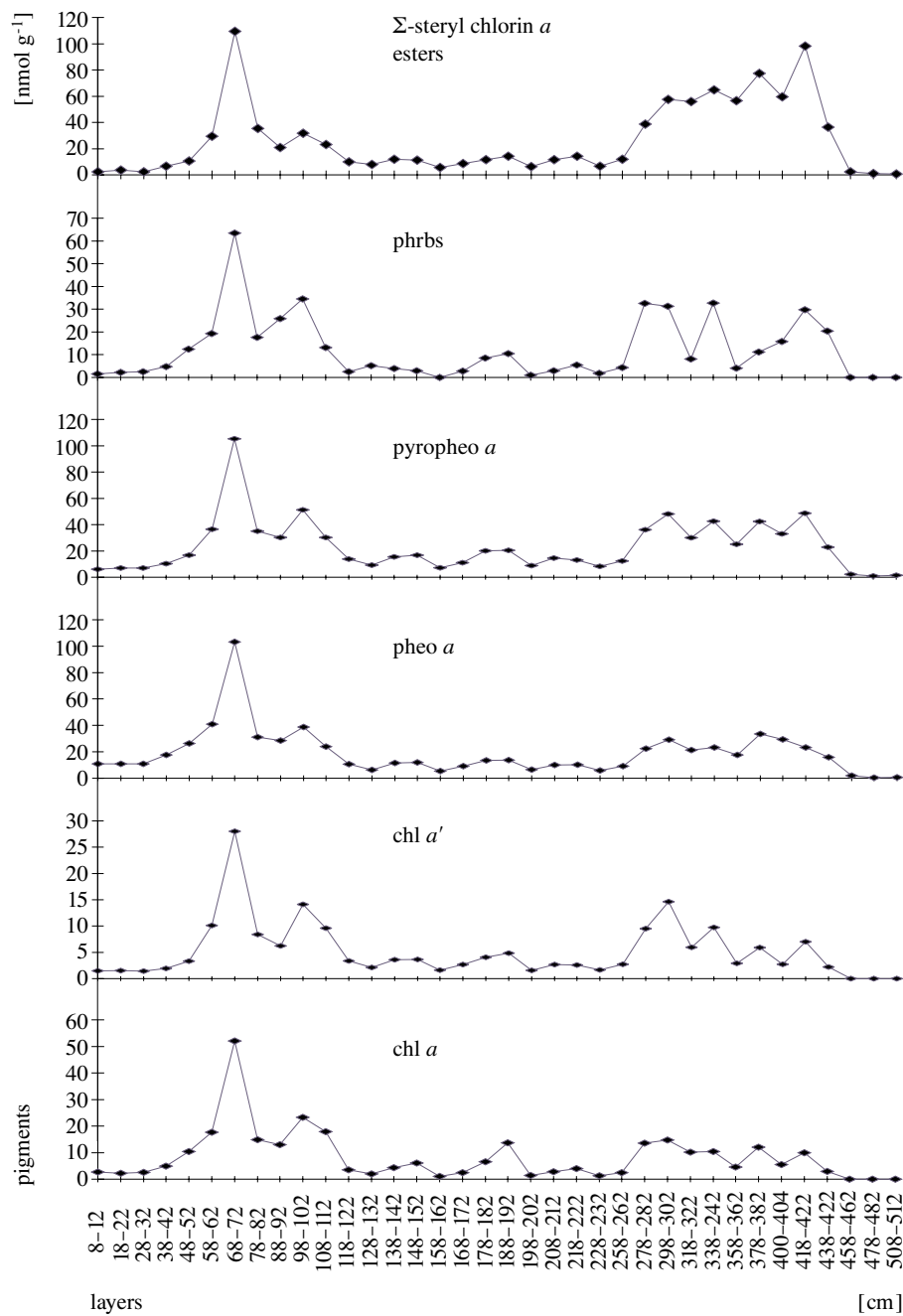
Fig. 6. Concentration profiles of chlorins a in the Gotland Deep sediment core: chl a – chlorophyll a , chl a' – chlorophyll a' (pyrochlorophyll a ), pheo a – phaeophytin a , pyropheo a – pyropheophytin a , phrbs (chlone) – phaeophorbides a -like (chlorophyllone epimers), steryl chlorin a esters – SCEs
