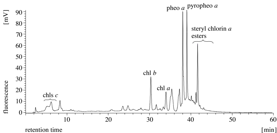
Fig. 5. Fluorescence HPLC chromatogram (Ex/Em – 440/630 nm) of a Gotland Deep sediment extract (layer 78–82 cm)
