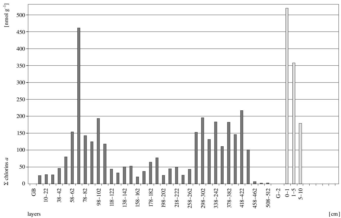
Fig. 8. Summed concentrations of chlorins a in the Gotland Deep (GB) sediments and recent (0–10 cm) sediments from the Gdańsk Deep (G-2) collected in March 1997
