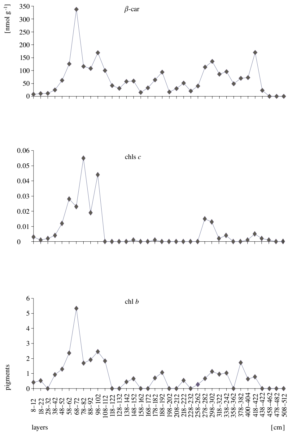
Fig. 7. Concentration profiles of chl b – chlorophyll b , chls c – chlorophylls c , \beta -car – \beta -carotene in the Gotland Deep sediment core
